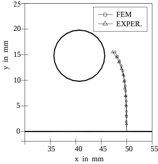
Figure 6 – Predicted and measured crack path.
