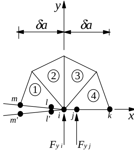
Figure 3 – Node at crack tip elements and consistent nodal forces ahead of crack tip.
