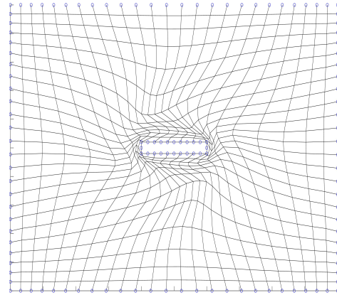
Figure 11: Final mesh using CTPS C^1 after 40 intermediate steps (test case 2).
