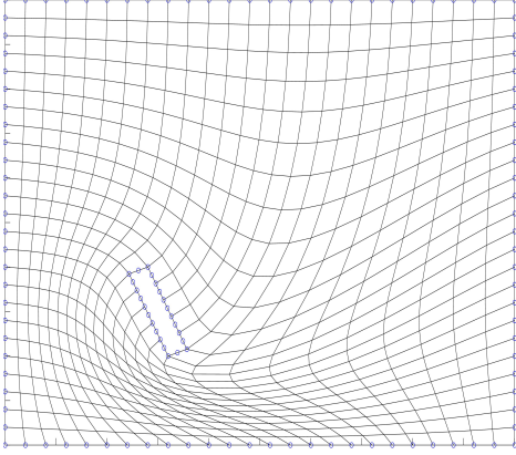
Figure 7: Final mesh using TPS with 15 intermediate steps (test case 1).
