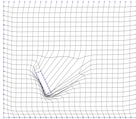
Figure 6: Final mesh using Gaussian basis function with 15 intermediate steps (test case 1).
