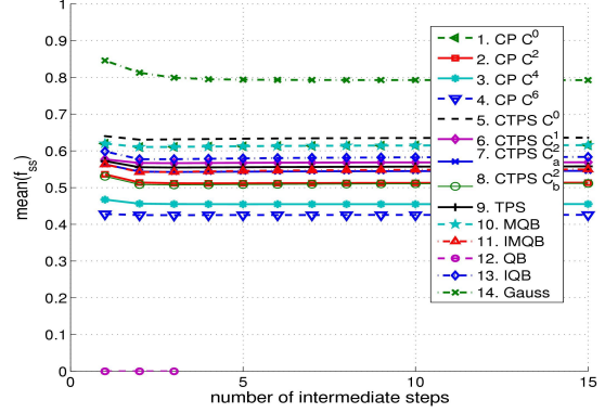
Figure 4: Average quality of the mesh for the different RBF's (test case 1).
