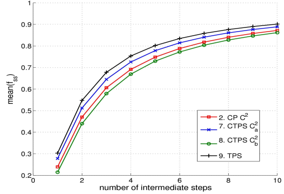
Figure 16: Average quality of the mesh for the different RBF's (test case 4).
