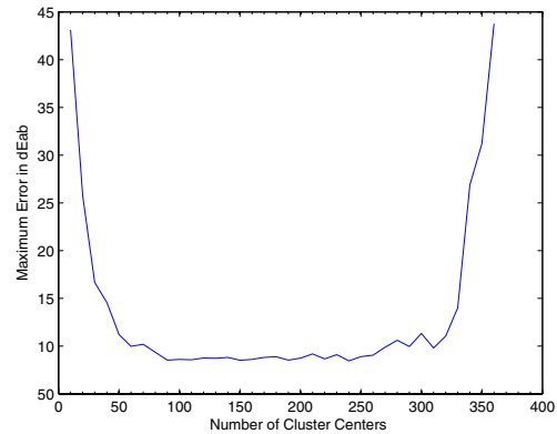
Figure 1. The maximum approximation error as a function of the number of centers in the RBF.
