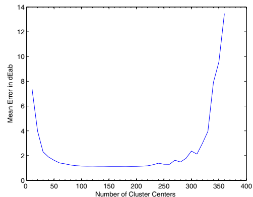
Figure 2. The average approximation error as a function of the number of centers in the RBF.
