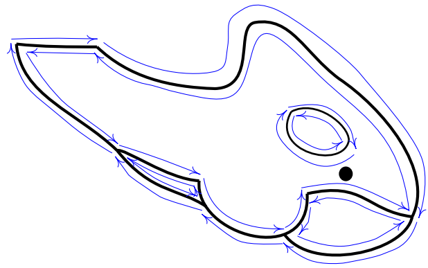
Figure 2: A doubly-connected edge list example.
